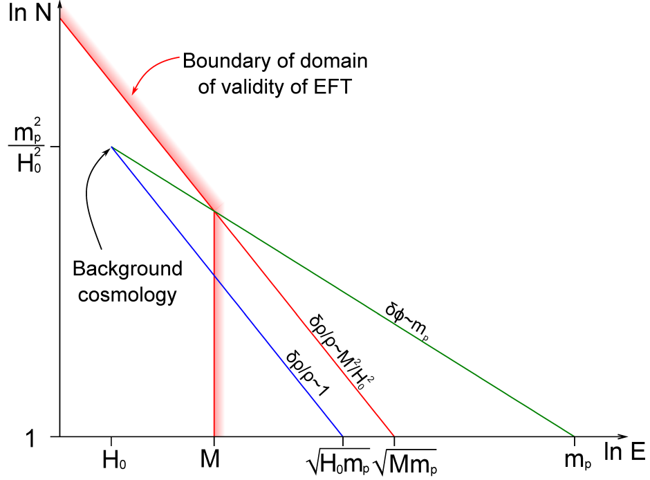
Figure 10: The domain of validity of the effective field theory in the two dimensional parameter space of energy E per quantum of a mode of the quintessence field, and mode occupation number N . The cutoff scale M must be larger than the Hubble parameter H_0 in order that the background cosmology lie within the domain of validity. Perturbation modes on length-scales that are small compared to H_0^{-1} but large compared to M^{-1} can be described, but only if the mode occupation number and fractional density perturbation are sufficiently small. See Section 4.5.II for details.
