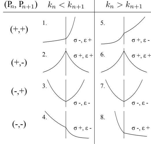
Figure 7: The behavior of the warp factor at a brane interface in the eight possible configurations. An increasing warp factor in a region has P_n = +1 , while a decreasing warp factor has P_n = -1 . In cases 2, 3, 6 and 7, the adjacent bulk cosmological constants can be equal. The horizontal axis in all plots is the y coordinate. Note that cases 2 and 6 are equivalent, for all intents and purposes, as are cases 3 and 7.
