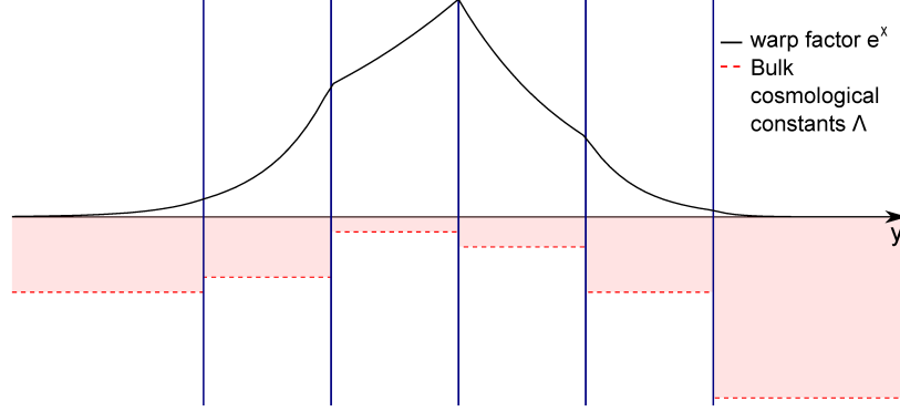
Figure 8: Diagram of a physically allowable warp factor between branes, and the associated bulk cosmological constants (dashed). Branes are represented as vertical lines. The bulk cosmological constants are negative, while the warp factor lies between 0 and 1.
