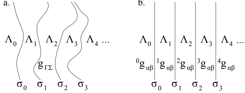
Figure 6: An illustration of the model a) before and b) after gauge fixing. The bulk cosmological constants, brane tensions, and metrics are labeled.
