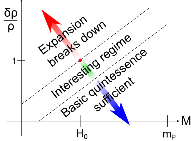
Figure 9: The parameter space of fractional density perturbation \delta\rho/\rho for perturbations to the quintessence field, and cutoff scale M for the effective field theory, illustrating the constraint (4.1.3) on the domain of validity. Near the boundary of the domain of validity the higher derivative terms in the action are potentially observable, this is labeled the “interesting regime”. Further away from the boundary the higher derivative terms are negligible and the theory reduces to a standard quintessence model with a matter coupling.
