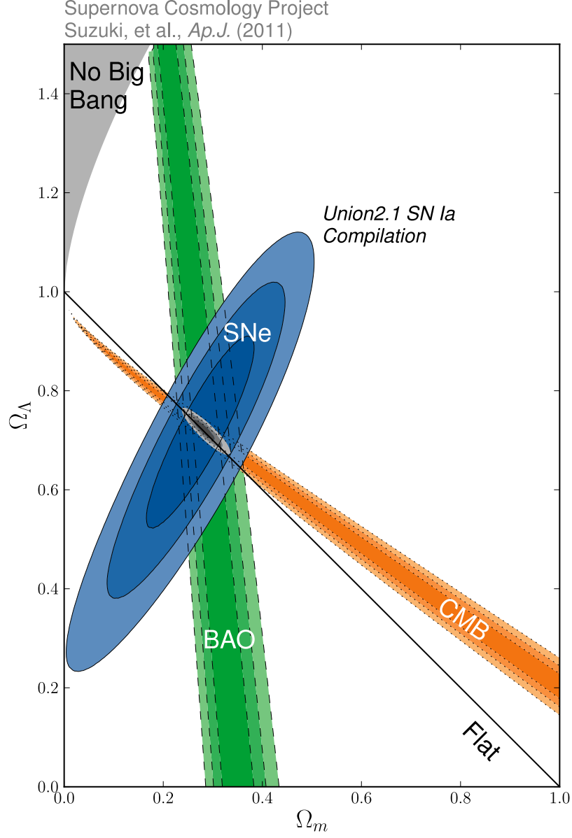
Figure 1: Constraints on the \Omega_\Lambda vs \Omega_{\text{matter}} plot, showing contributions from the cosmic microwave background, Type Ia supernovae, and baryon acoustic oscillations (excluding systematic errors). Note that the three methods are highly complementary. Figure from Ref. [13]. Reproduced by permission of the AAS.
