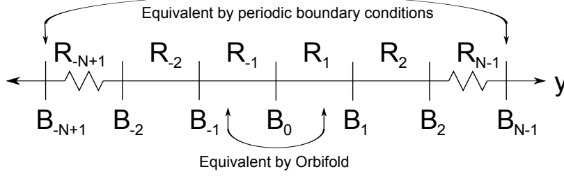
Figure 11: Diagram indicating how the branes are labeled in the construction of the orbifolded model. The orbifold symmetry identifies y with -y , and we impose the periodicity condition of identifying y with y + 2N - 2 . To calculate the action, the model is broken up into 2(N - 1) bulk regions \mathcal{R}_n , but regions \mathcal{R}_n and \mathcal{R}_{-n} coincide by the orbifold symmetry.
