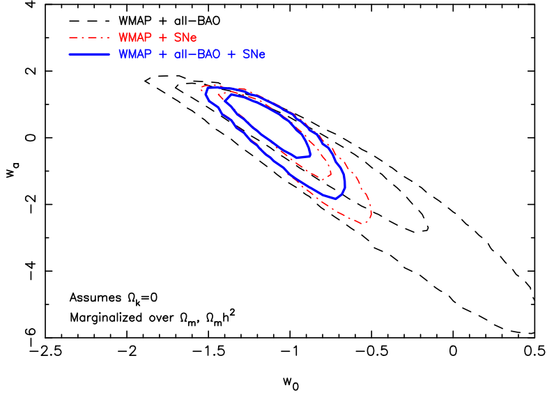
Figure 5: Current constraints on the equation of state of dynamical dark energy, using the parametrization given in Eq. 1.2.1. Figure from Ref. [17]. Reproduced by permission of John Wiley and Sons.
