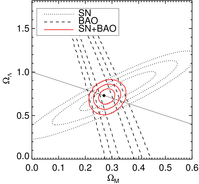
Figure 3: Recent constraints on the \Omega_\Lambda vs \Omega_{\text{matter}} plot, comparing results from Type Ia supernovae and baryon acoustic oscillations. Figure from Ref. [15]. Reproduced by permission of the AAS.
