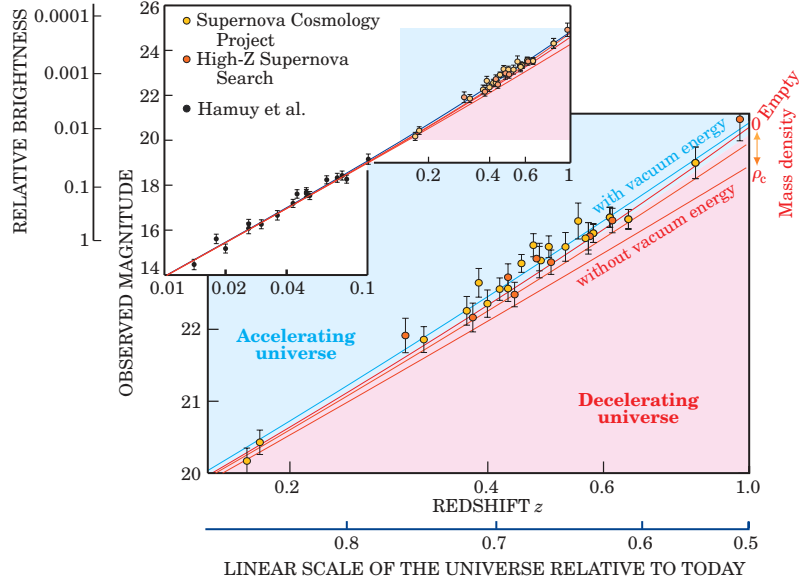
Figure 2: Luminosity of observed Type Ia supernovae plotted against redshift, including a comparison to dependence on expansion history of the universe. Figure from Ref. [14]. Reprinted by permission of the AIP.
