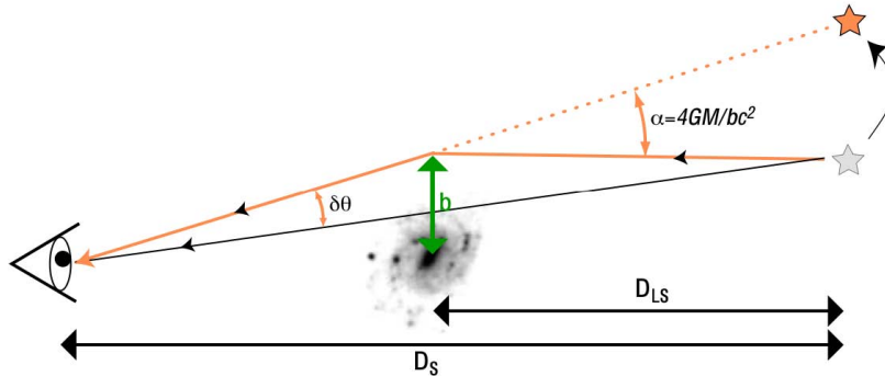
Figure 4: Diagrammatic overview of weak lensing phenomenon. Figure from Ref. [16]. Reproduced by permission of authors.
